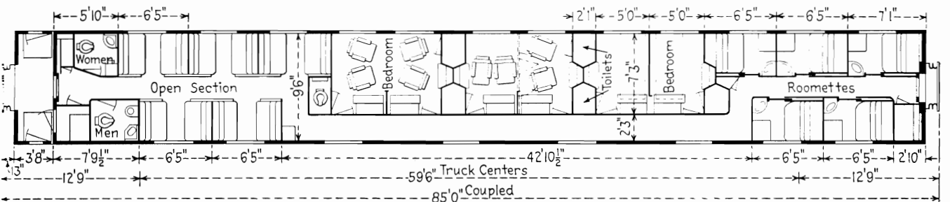
Floor plan of Denver & Rio Grande Western sleeping car having 6 bedrooms, 5 roomettes and 5 open sections. Builder, Pullman-Standard Car Manufacturing Co.
