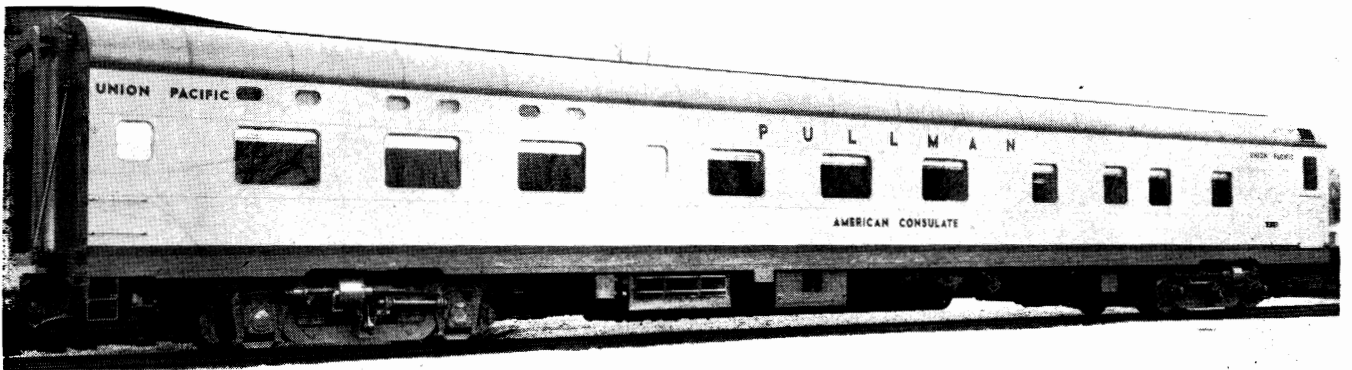
Exterior and floor plan of sleeping car having 6 sections, 6 roomettes and 4 bedrooms. Builder, American Car and Foundry Co.
